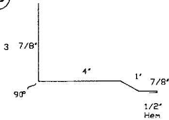
Universal Sidewall
