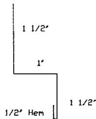
Double Angle
