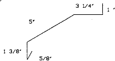
Top Mount Track Cover
