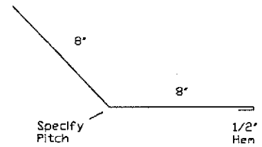
Transition Flashing
