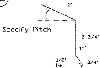
Denver Eave
