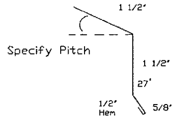
Residential Drip Edge
